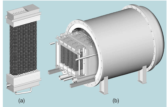
Fig. 4 Structure of (a) cartridge and (b) pressurized module Cartridge type superior in reliability and extendability is adopted as the module.
