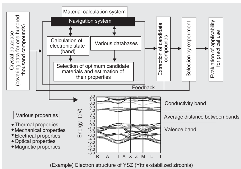
Fig. 13 Flowchart of development of top coat material, utilizing first principle band calculation
