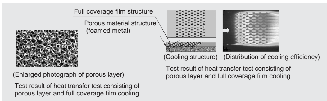
Fig. 7 Example of transpiration cooling system
