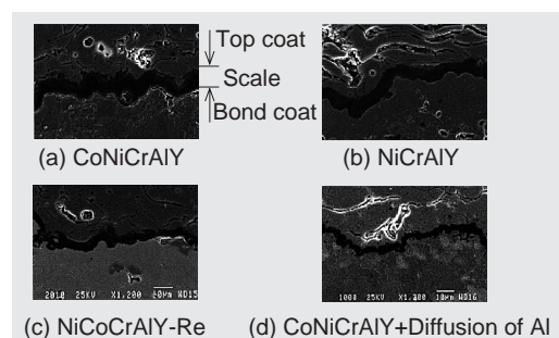
Fig. 15 Observation results of oxide scales after oxidation test of various bond coats ( 1000^{\circ}C \times 1000 h )
