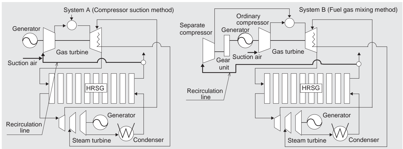
Fig. 2 Recirculation system
