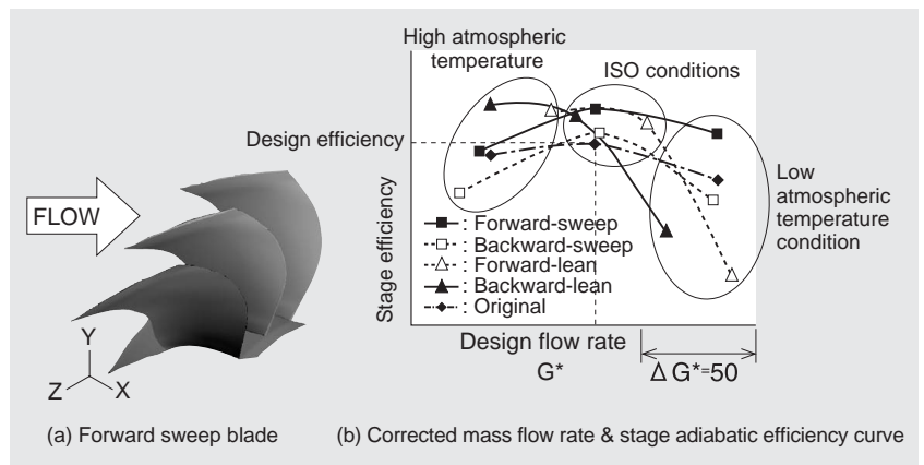
Fig. 19 Investigation of three-dimensional blade
