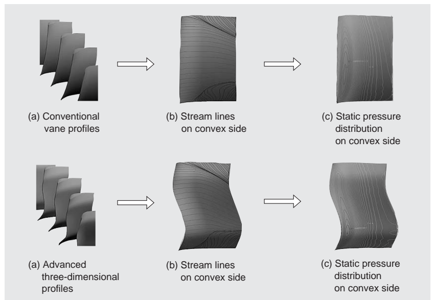
Fig. 20 Comparison between conventional stationary vane and newly designed three-dimensional stationary vane
