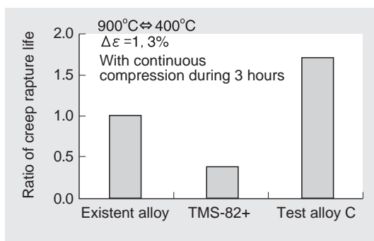
Fig. 10 Thermal fatigue test result for each alloy
