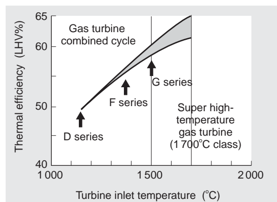
Fig. 1 Relationship between turbine inlet temperature and combined efficiency
