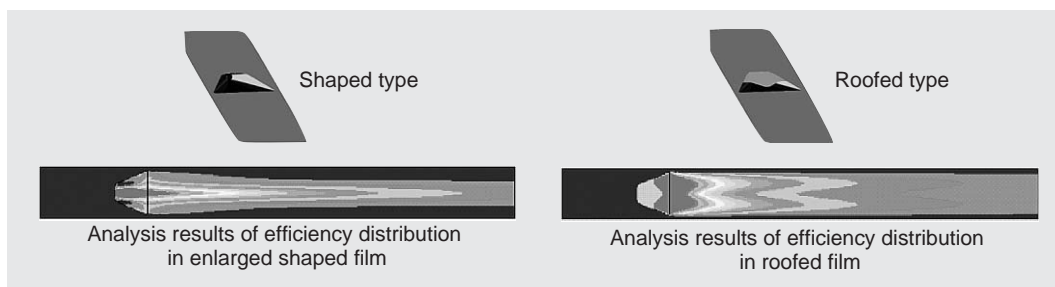
Fig. 8 Analysis result of new type film cooling
