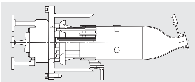
Fig. 3 Examination schematic of 1700°C diffusion type combustor
