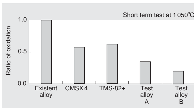
Fig. 11 Atmospheric oxidation test results for each alloy
