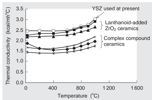
Fig. 14 Results of measurements of thermal conductivity of trial manufactured sintered ceramics
