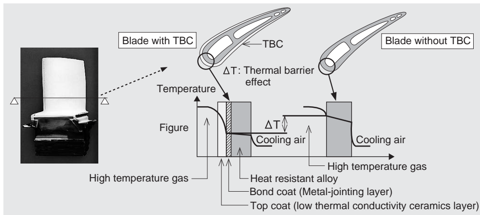
Fig. 12 Thermal barrier effect of TBC
