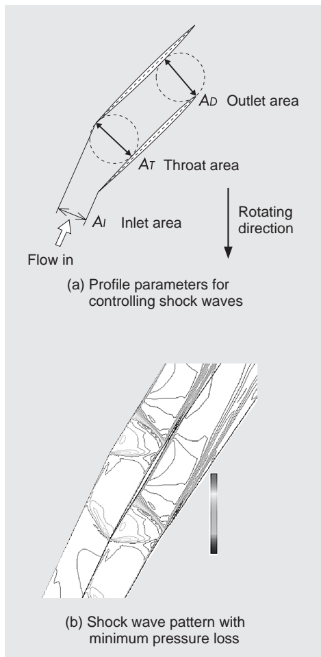
Fig. 18 Pattern of shock waves with minimum pressure loss
