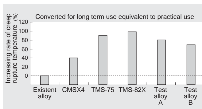
Fig. 9 Comparison of improvement in creep rupture temperature for each alloy
