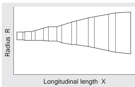
Fig. 16 Profile of turbine flow path
