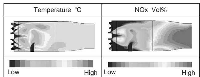
Fig. 4 Virtual images of temperature distribution and NOx concentrations by CFD in diffusion type combustor
