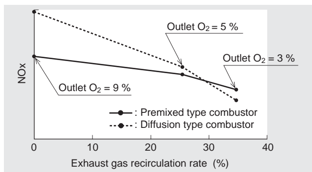
Fig. 5 Estimation of emitted NOx by CFD
