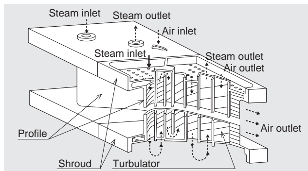
Fig. 6 Conceptual view of cooling system of first stage stationary vane of turbine
