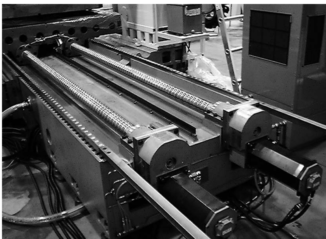
Fig. 1 X-axis twin ball screw Indicates two pieces of ball screw installed at the rear end of the bed.
