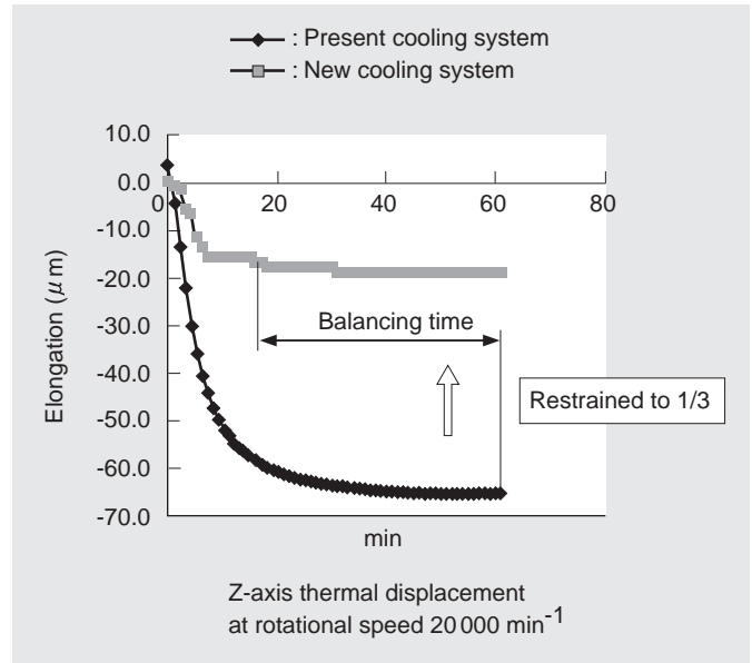
Fig. 2 Thermal displacement of main spindle in Z-axis direction
