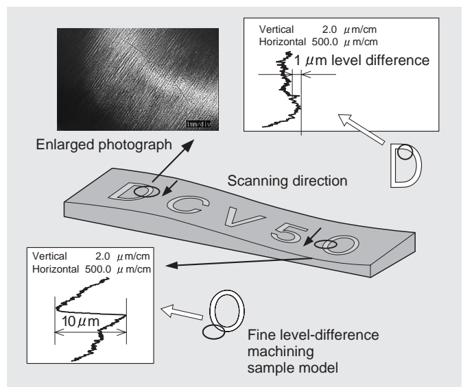
Fig. 4 Micro-machining level-difference sample cutting
