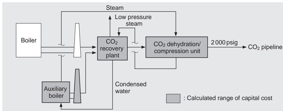
Fig. 2 Boiler case
