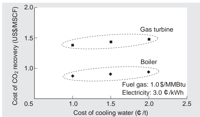
Fig. 6 Relation between CO 2 recovery cost and cooling water cost
