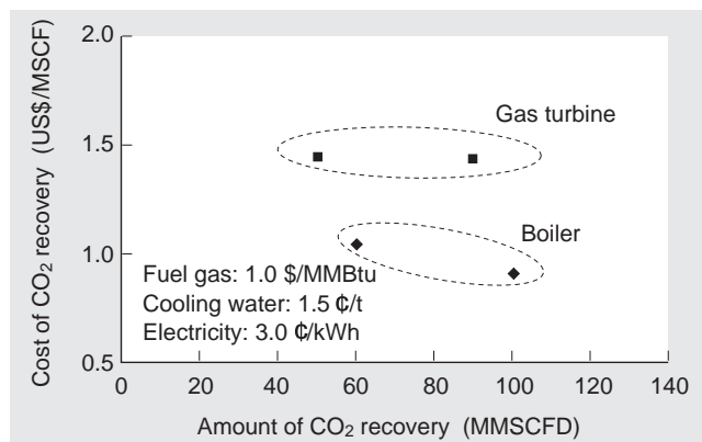
Fig. 4 Relation between CO 2 recovery cost and CO 2 recovery capacity in the flue gas CO 2 recovery plant
