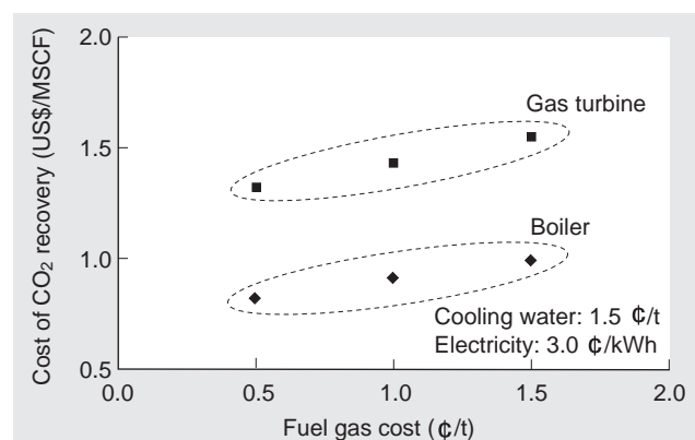
Fig. 5 Relation between CO 2 recovery cost and fuel gas cost
