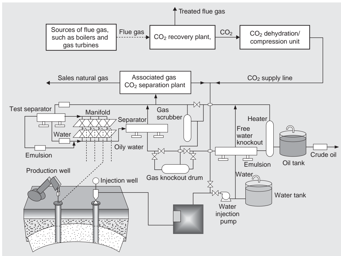
Fig. 1 Concept of overall system for CO 2 EOR
