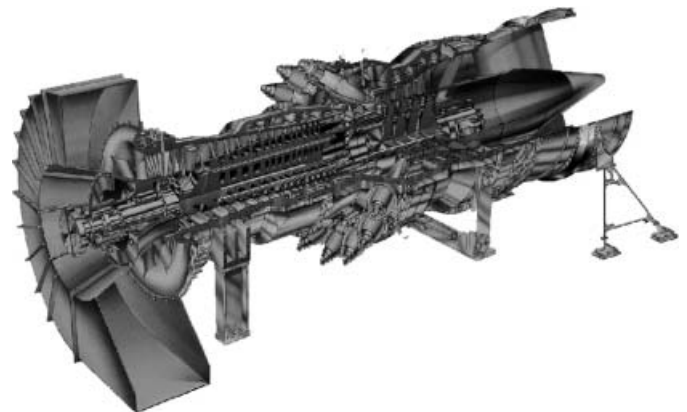
Fig. 3 M501F gas turbine Up-rated M501F gas turbines are used in all combined-cycle power plants delivered by MHI in Mexico.
